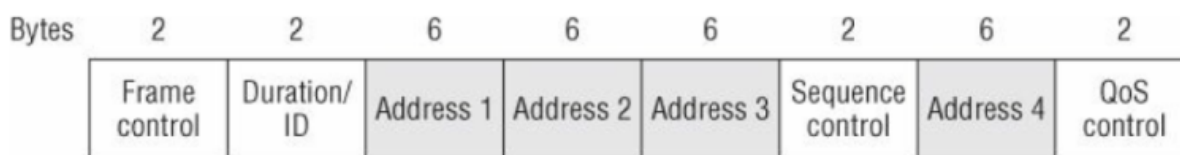
Figure 9.3 802.11 MAC header
